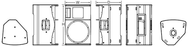
Dimension(W×H×D):446×700×440mm
